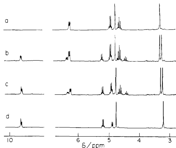
Figure 1. 1 H NMR spectral changes occurring during the hydrolysis of a 0.1 M solution of acetaldehyde cis -1-propenyl methyl acetal in 0.001 M DCl/D 2 O. Spectra measured at 200 MHz and ambient temperature: (a) substrate in D 2 O; (b) after adding DCl; (c) 15 min later; (d) next day.
